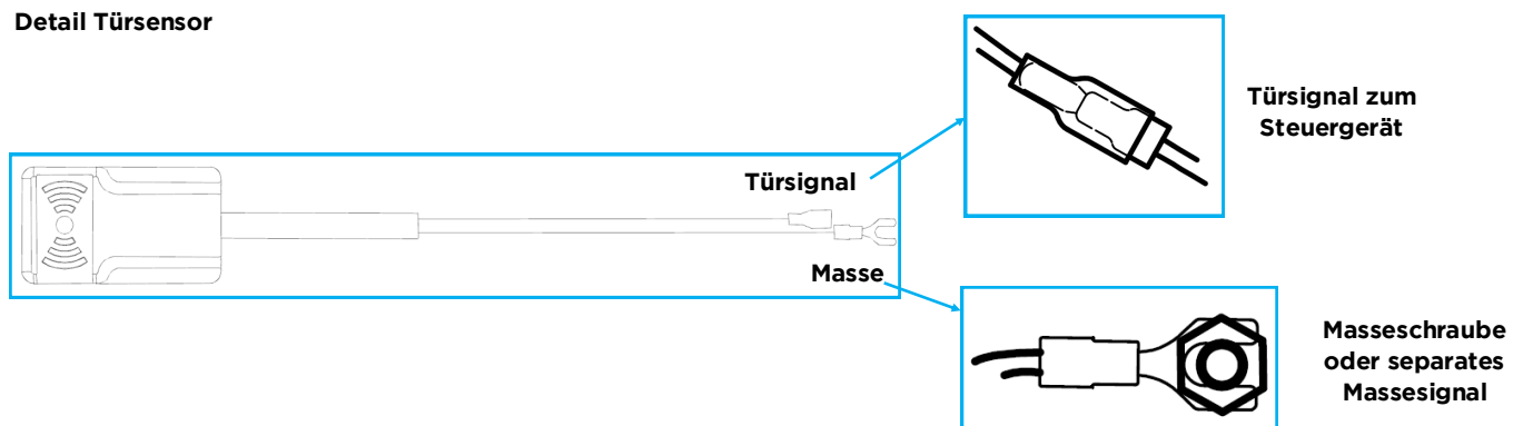
Detail Türsensor
