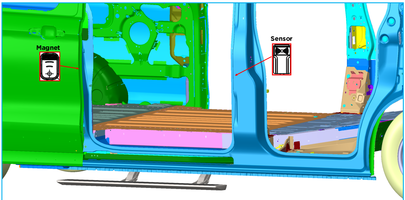
Detail Türsensor
